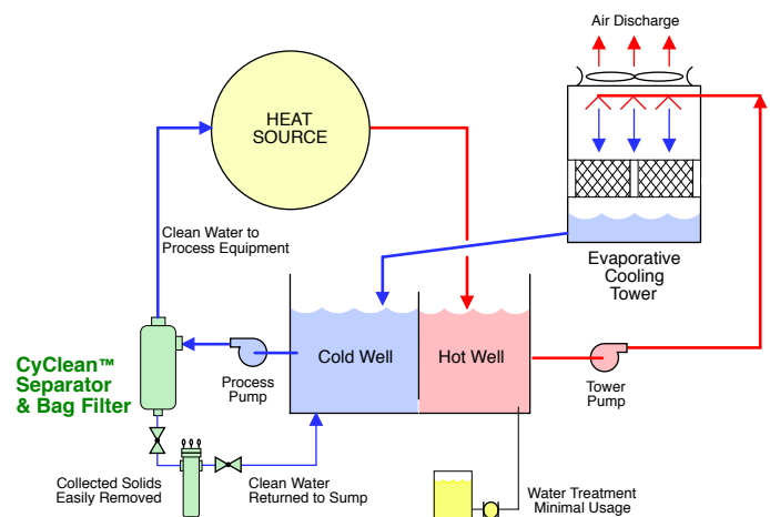
Typical Process Diagram
