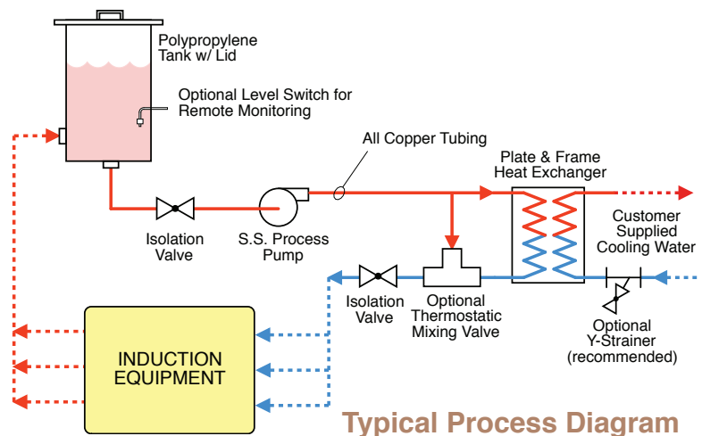
The Aqua-Vent® NFP-80 Non-Ferrous Cooling System with Thermostatic Mixing Valve and Tank Level Switch. Designed to provide 35 gpm at 80 psi and a cooling capacity of 80 kW.
